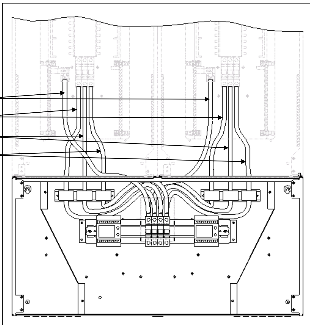
Diagram a. Cable connections.
