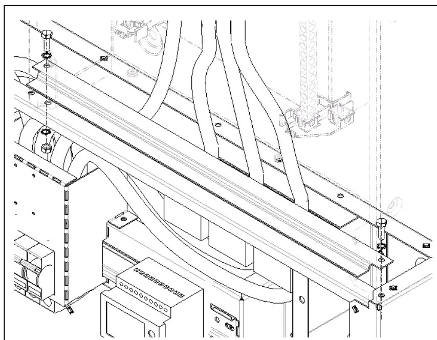
Diagram b Cross strap fixing
