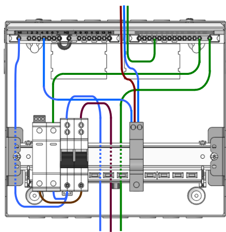
Fig 4.2 – connection to RCBOs/AFDDs (1 Mod)
