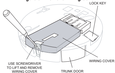
Figure 5 – Remove Wiring Cover
