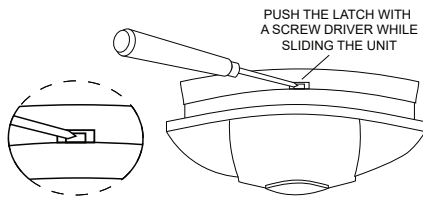
Figure 4 – Release Temporary Lock
