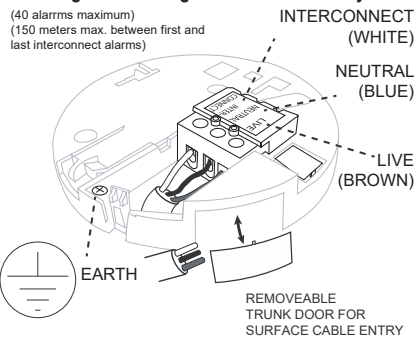
Figure 6 – Wiring & Interconnect facility
