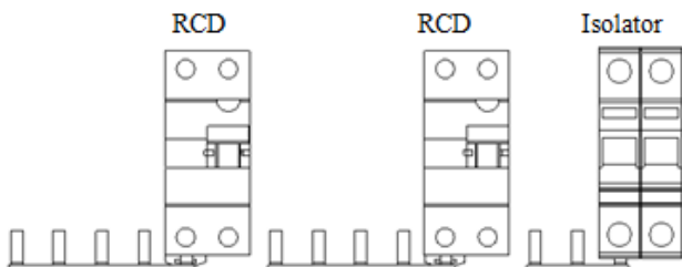
Illustration of a typical busbar fitting arrangement for a High Integrity unit
